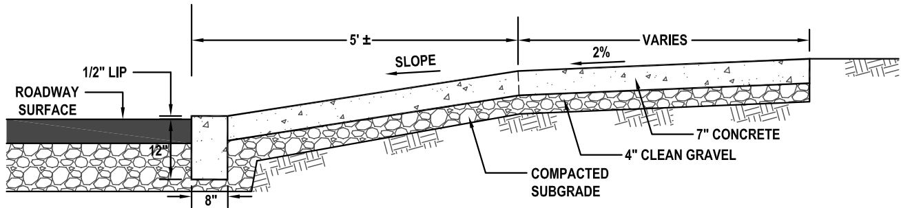
SECTION
