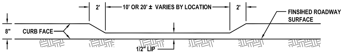
CURB FACE ELEVATION
