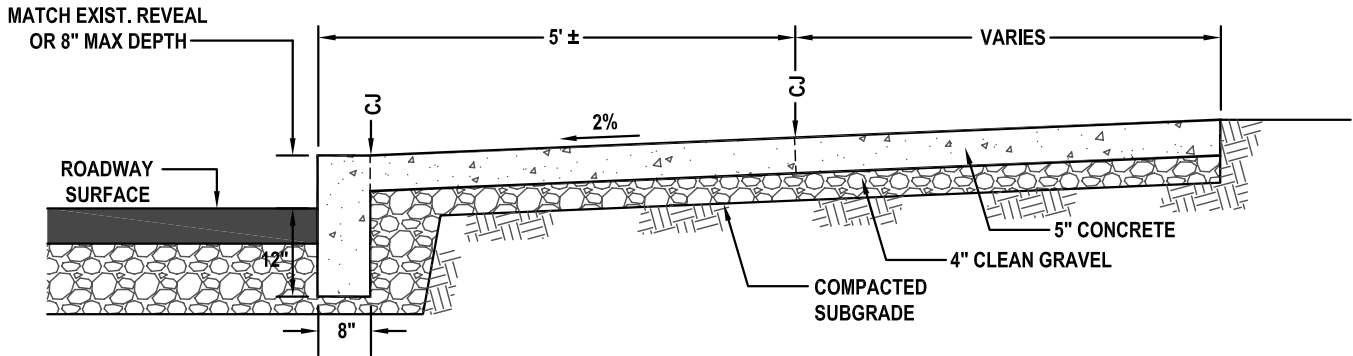
SECTION MONOLITHIC CURB & 5" SIDEWALK
