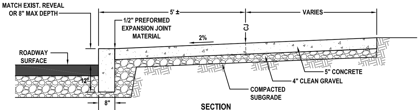
SECTION STRAIGHT 8" CURB W/ 5" SIDEWALK
